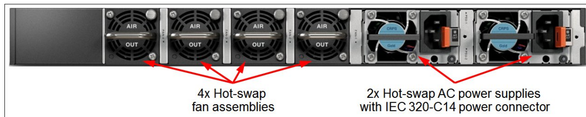
Figure 3. Rear panel of the RackSwitch G8272
