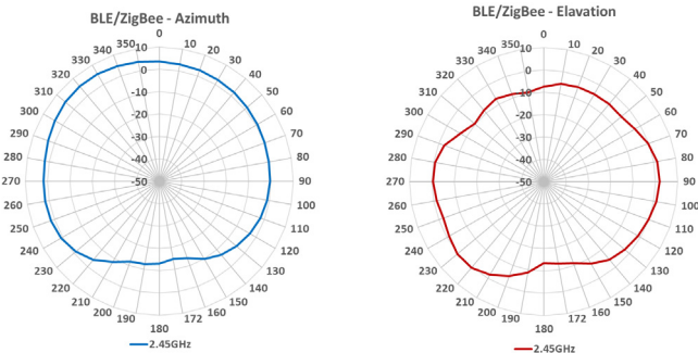
BLE/ZigBee Plot
