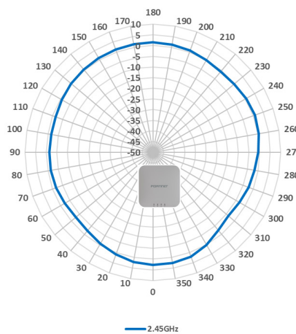
BLE/ZigBee Azimuth
