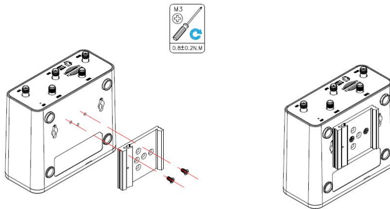
Horizontal installation
