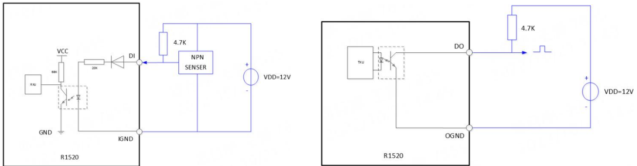
DI&DO Typical Connection Diagram
